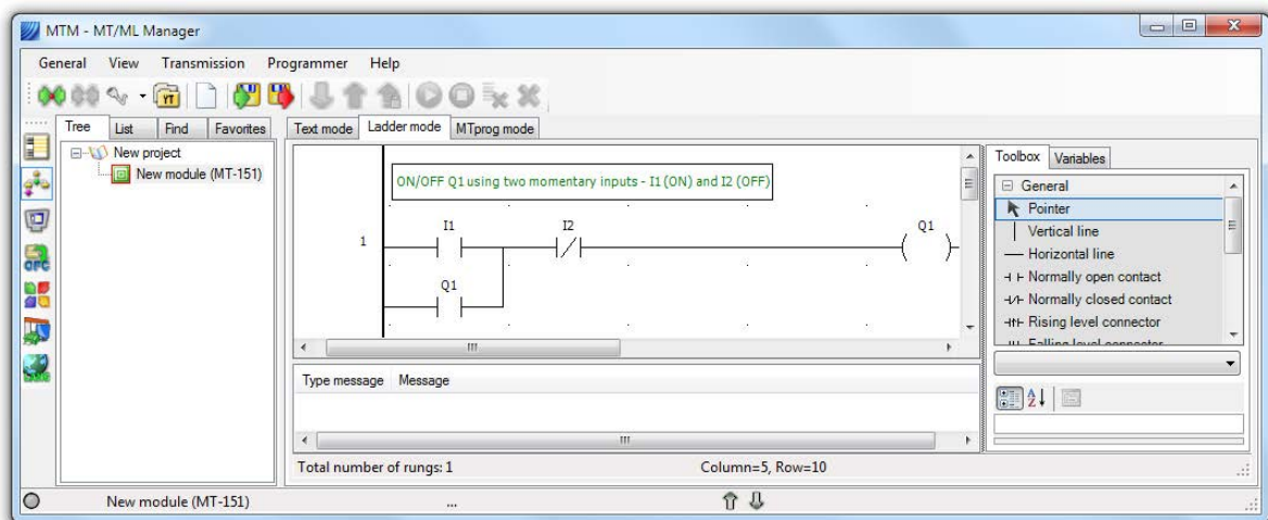
MTManager - sample program in ladder mode
