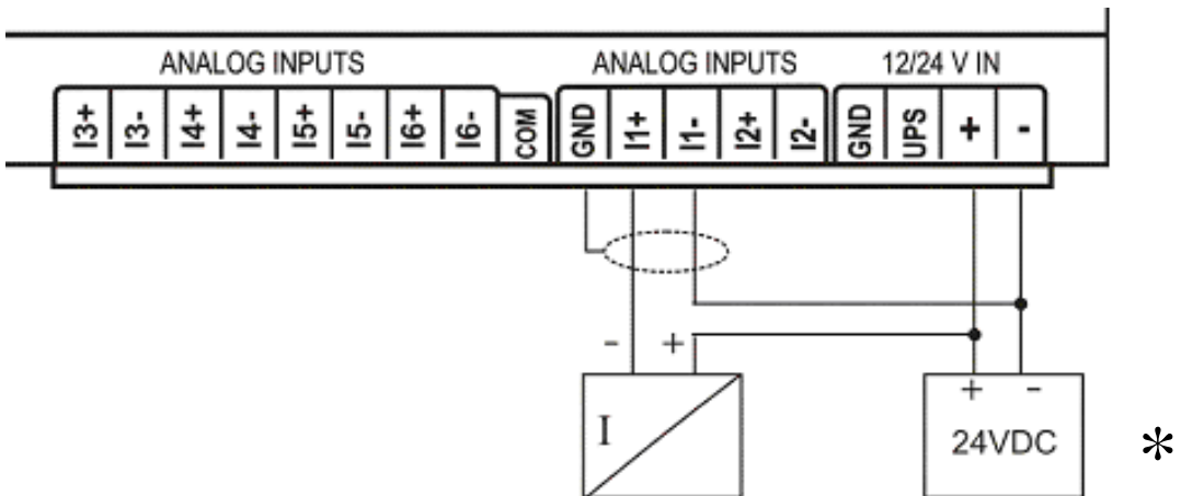
Analogue inputs A1...A6 – connection with passive output converter
