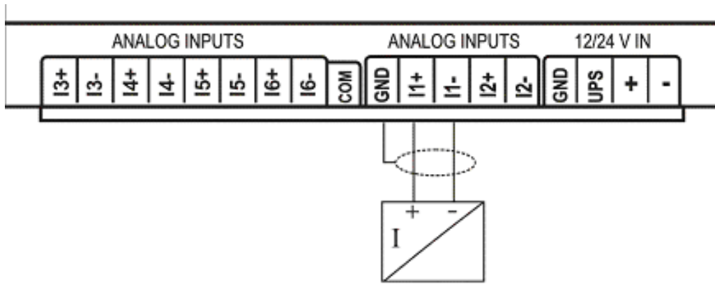
Analogue inputs A1...A6 – connection with passive output converter
