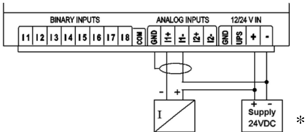
Analogue inputs A1 , A2 – connection with passive output converter
